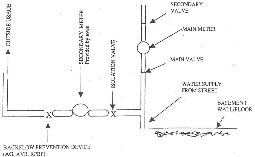
Typical Detail of Secondary Meter Installation
