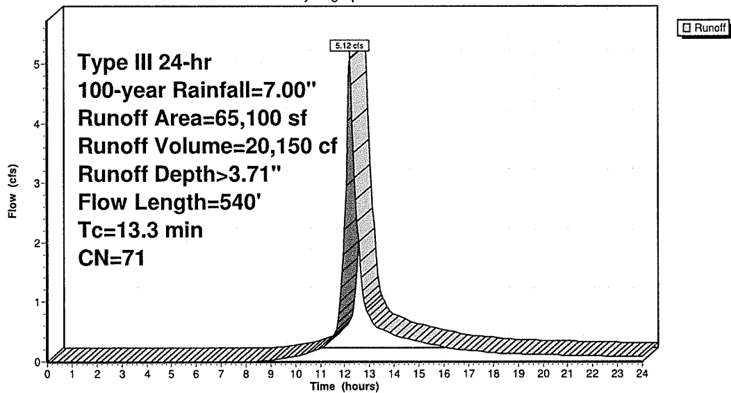
Hydrograph
