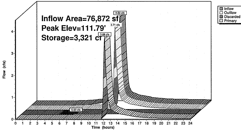
Hydrograph
