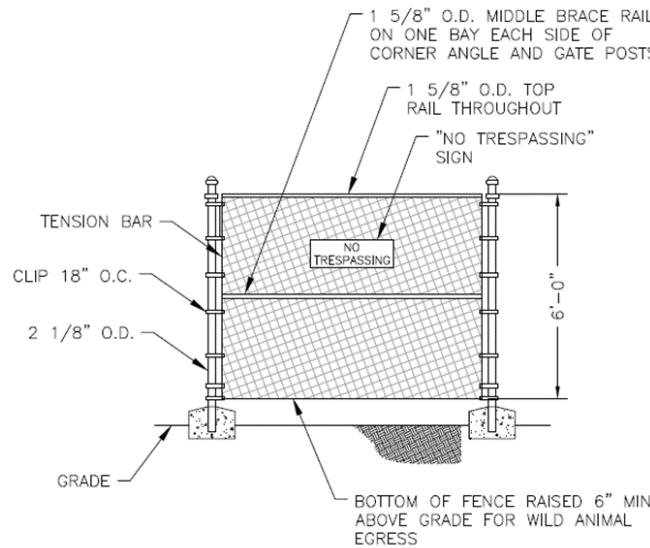
PERIMETER FENCE DETAIL NOT TO SCALE
