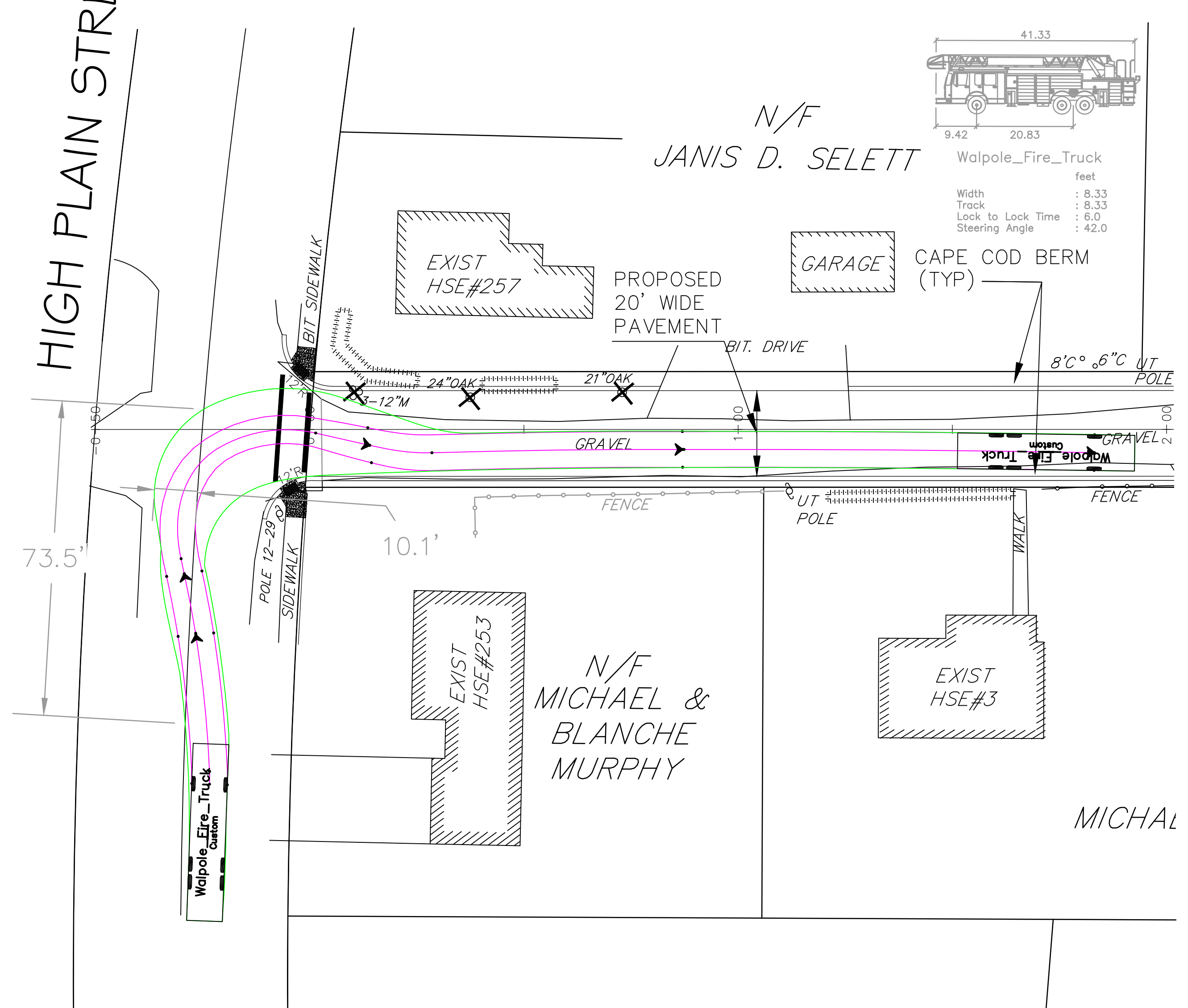
FIRE APPARATUS TURNING MOVEMENTS
