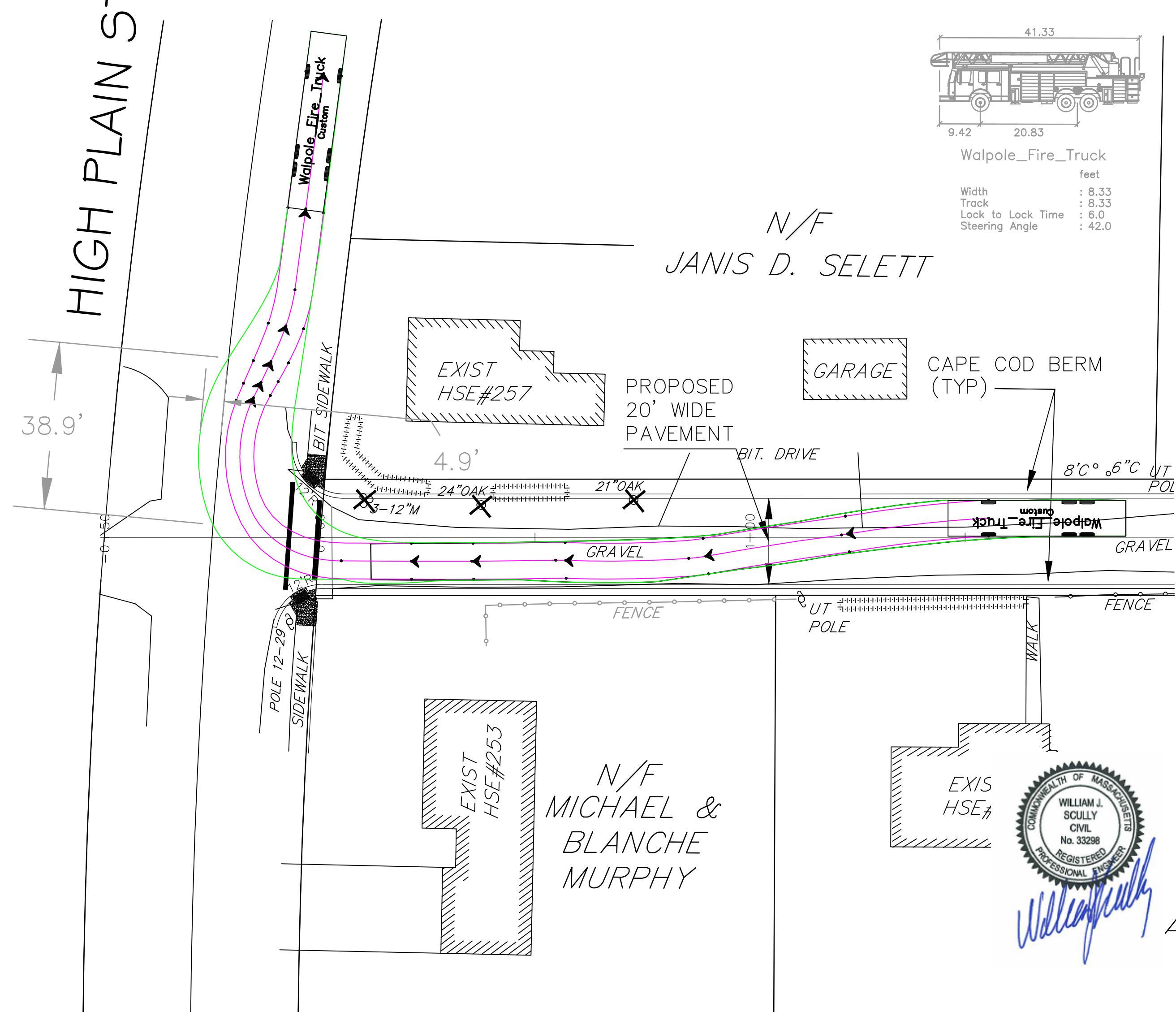
FIRE APPARATUS TURNING MOVEMENTS
